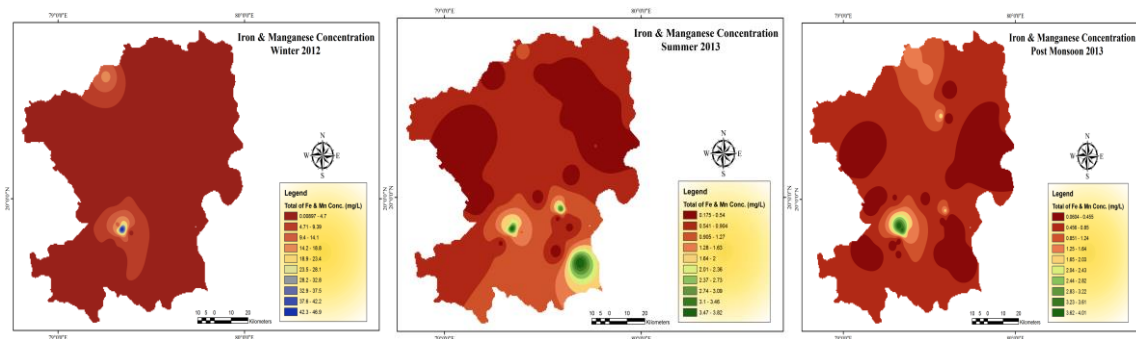
(a) Winter (b) Summer (c) Post-monsoon Figure 6: Spatial variation maps showing groundwater iron and manganese combined concentration of the study area
