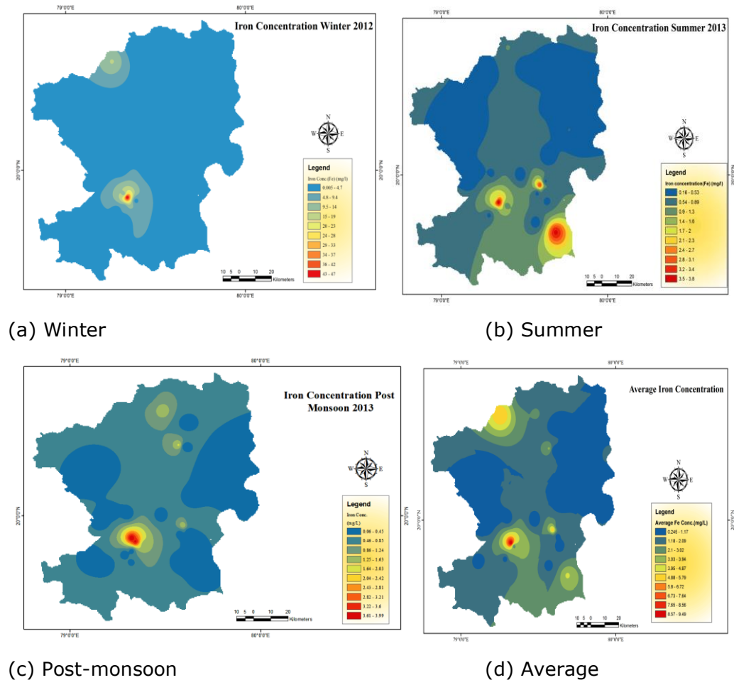
Figure 4: Spatial variation maps showing groundwater iron concentration of the study area
