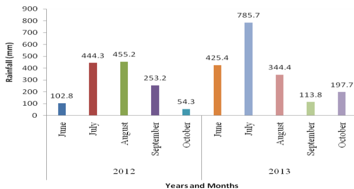
Figure 3: Rainfall during the study period (in mm)
